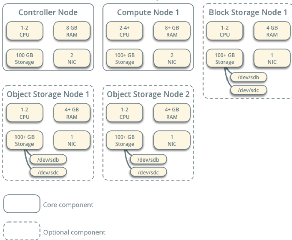
Fig. 1: Hardware requirements
