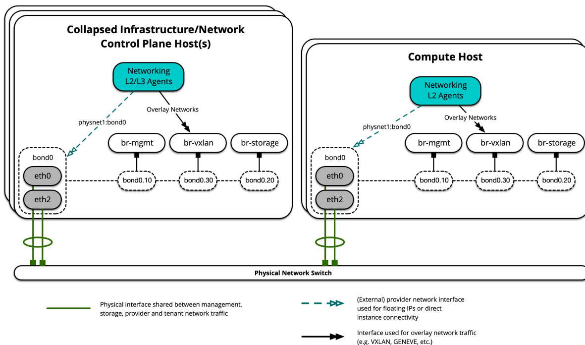
Network Interface Layout - Single Bond
