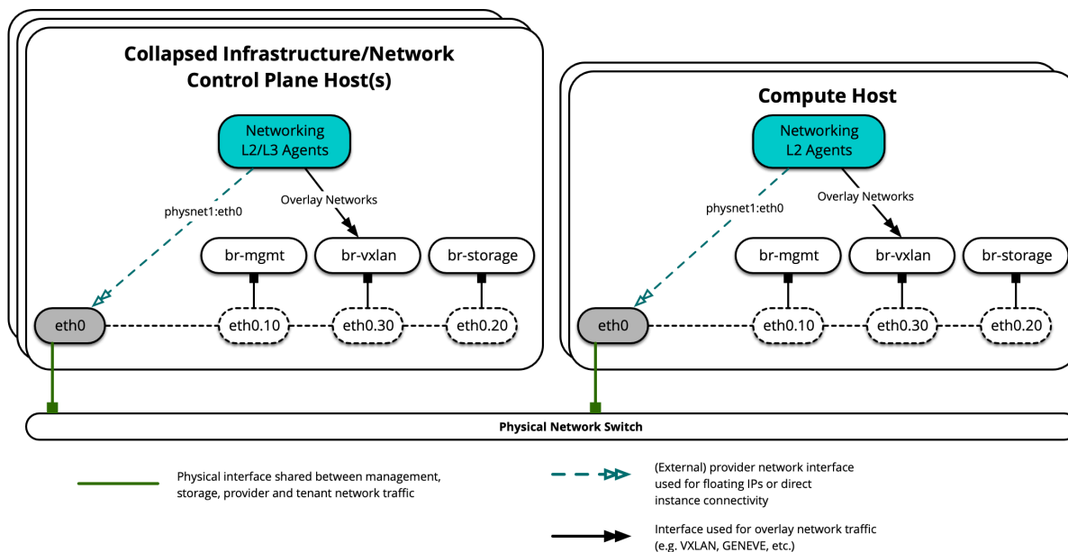
Network Interface Layout - Single Interface
