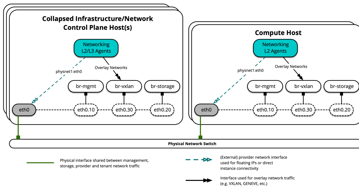
Network Interface Layout - Single Interface
